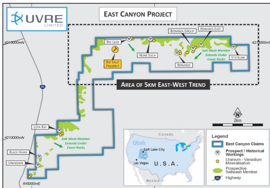
Figure 4. East Canyon project showing 5km East-West Trend to the east of the 5km East-West Trend, the Stateline prospect returned high scintillometer readings with carnotite and uraninite or coffinite observed (picture 2) within crumbly clay stone close to a sandstone contact.
