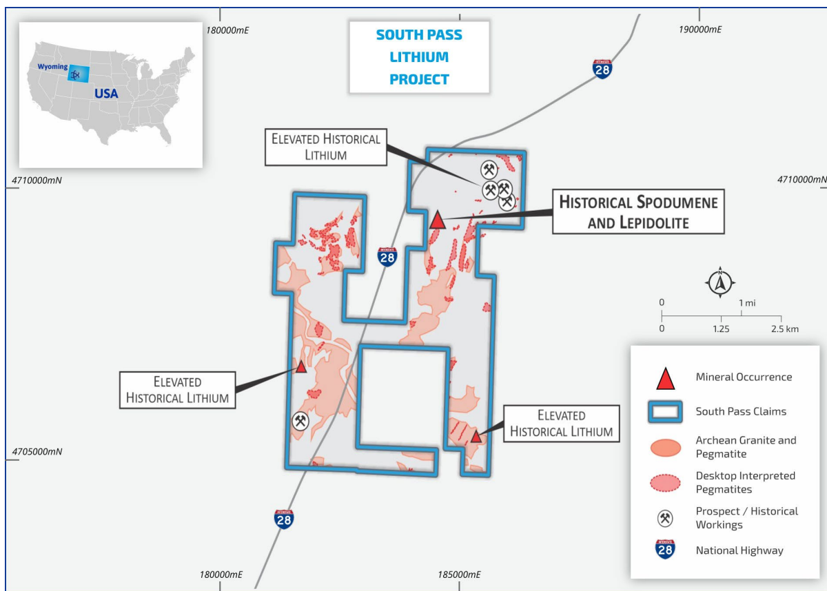
Figure 6. South Pass Lithium Project geology map showing spread of Archean granites and pegmatites.
