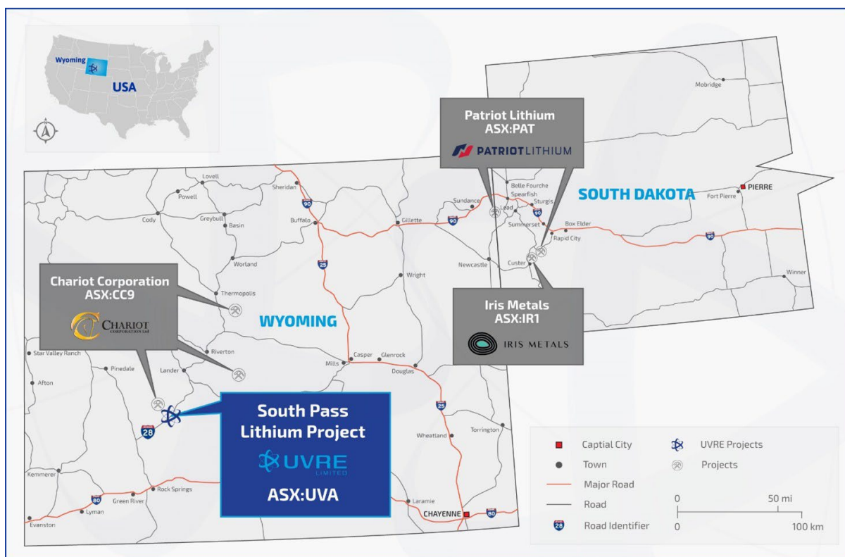
Figure 5. Location of South Pass Project in emerging Wyoming-South Dakota lithium province.
