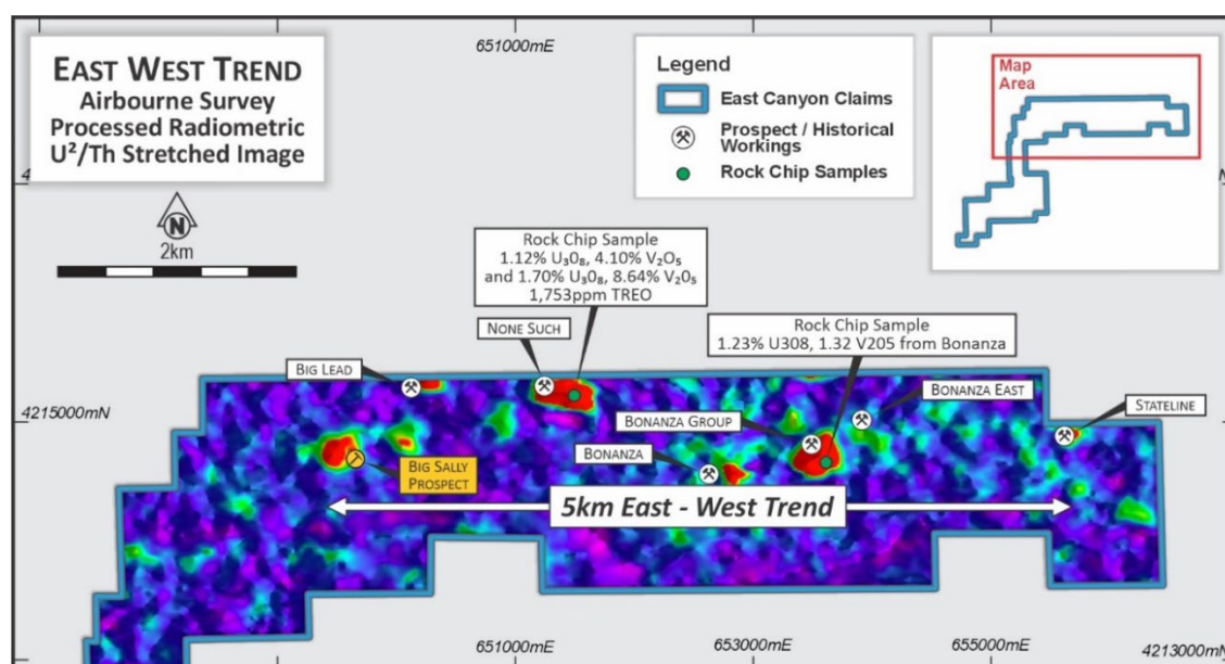
Figure 3: 5km East-West Trend image of the processed radiometric data showing the U^2/Th ratio imagery which has been stretched to identify the highest tenor areas of interest in which to focus exploration for uranium. The newly identified anomaly Big Sally in the western portion of the trend was previously unknown and is untested.
